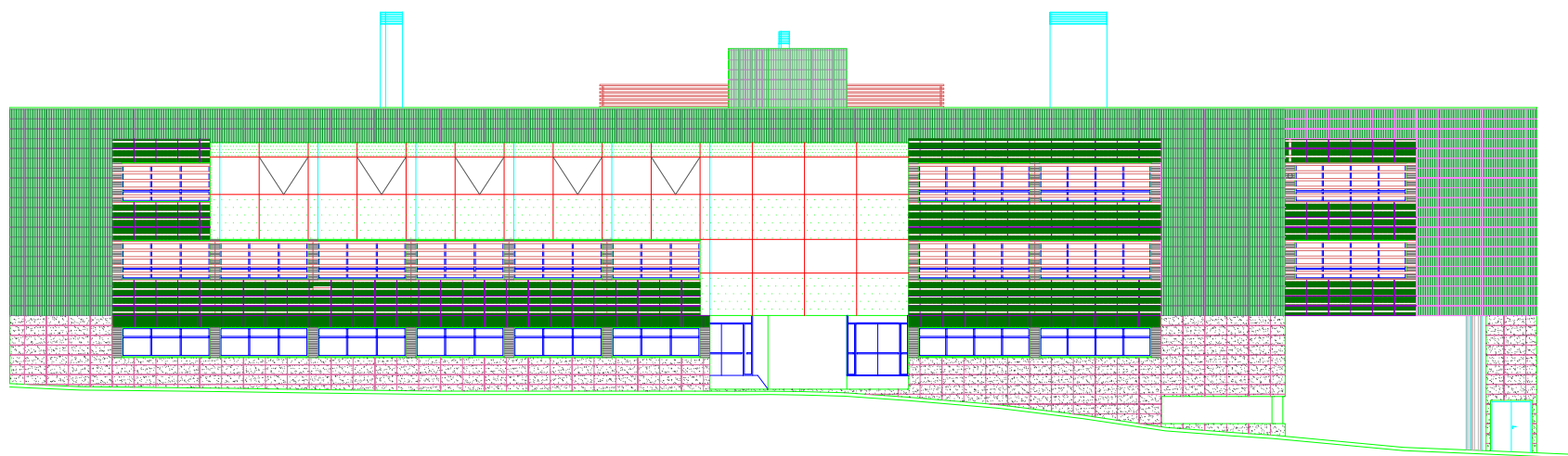
Alzado Principal
